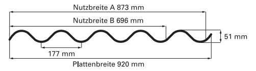
Profil 177/51 - P5 - PVC
